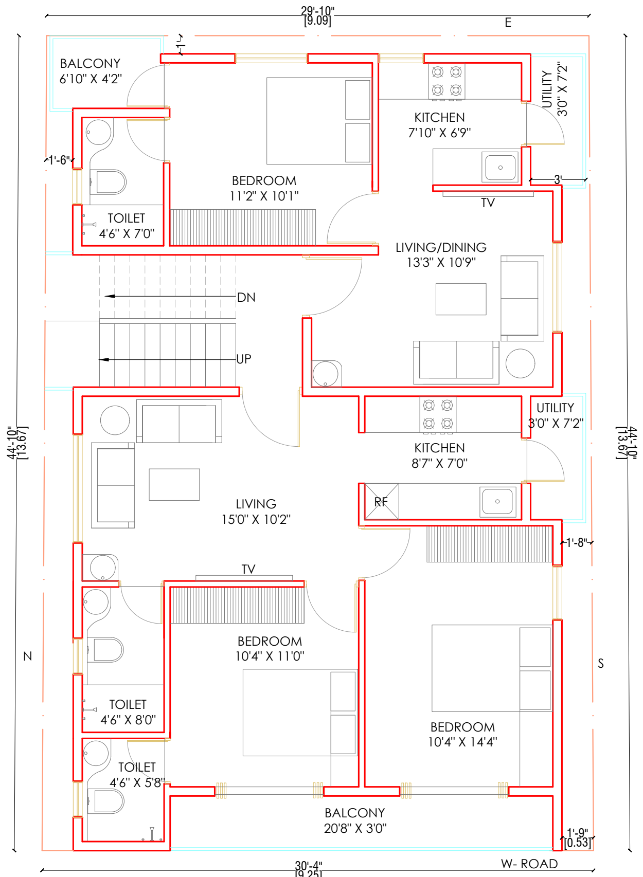
FIRST FLOOR PLAN:- 1089 SFT BALCONIES & UTILITIES:- 130 SFT
